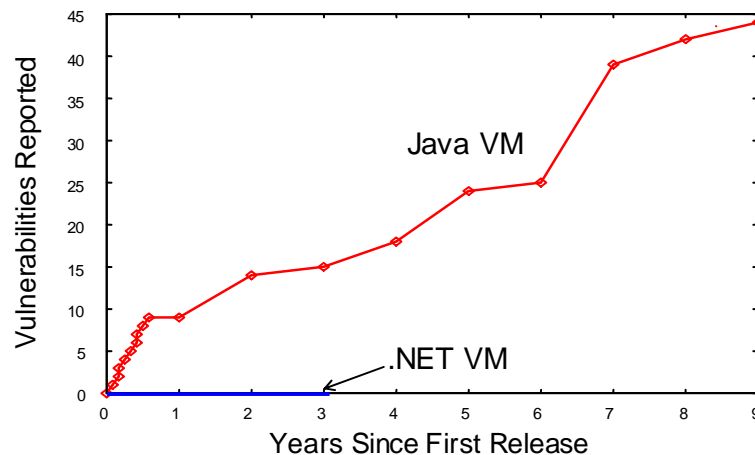
Figure 1. Major security vulnerabilities reported. The value plotted is the cumulative number of security vulnerabilities reported in each platform since the first official release (Java 1.0 in January 1996 [40]; .NET 1.0 in January 2002 [26]).
